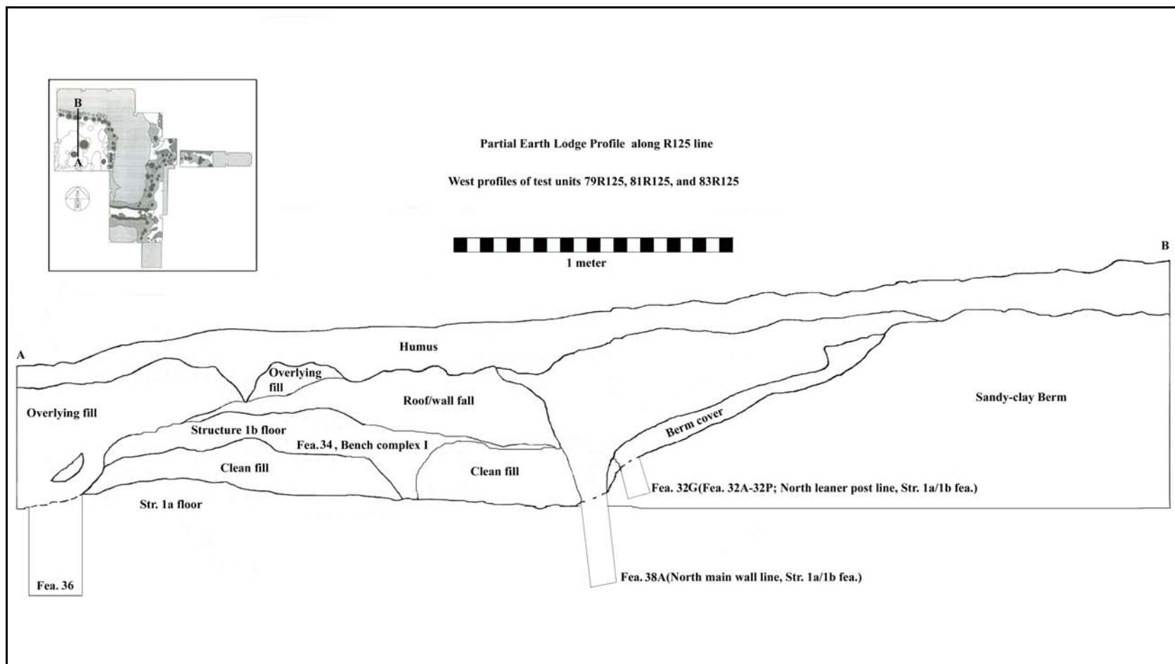
Figure 2.2. Partial earth lodge profile with stratigraphic deposits and certain features labeled.
